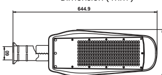
Dimension ( mm )
