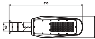
Dimension ( mm )
